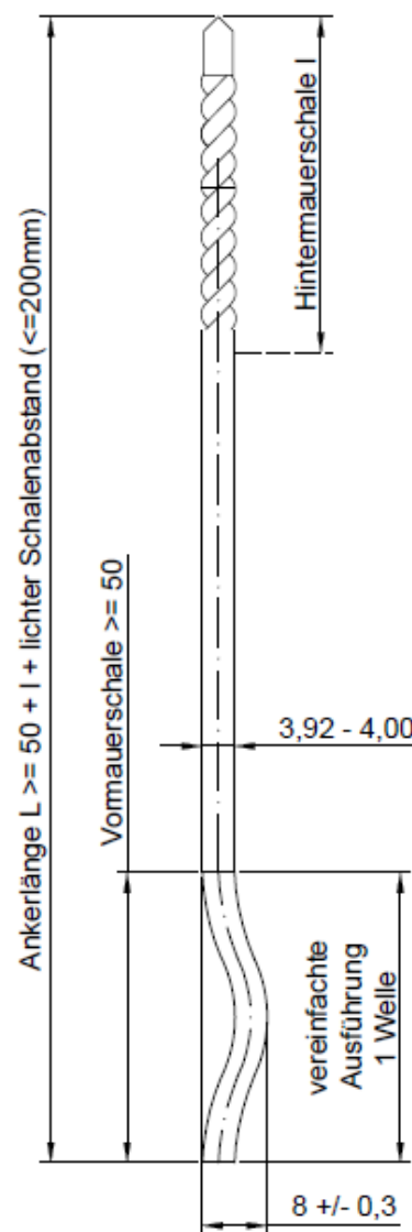
"Well-L-Form" (1 Welle)
