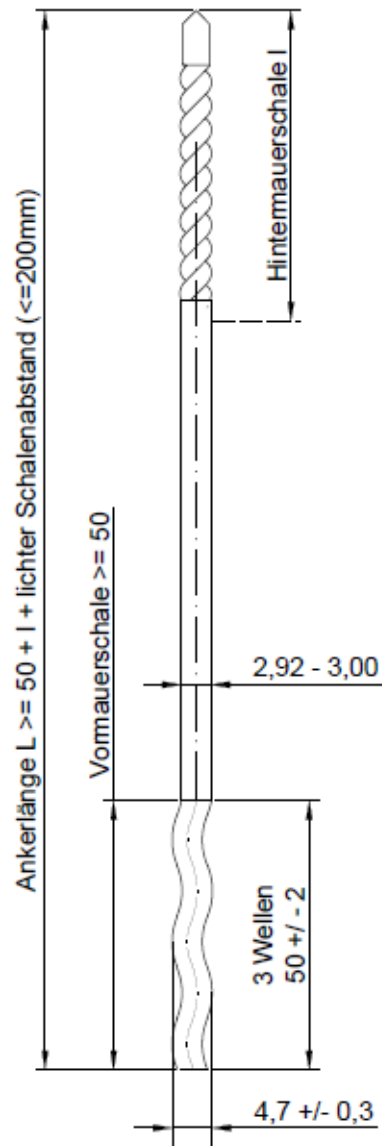
"Well-L-Form" (3 Wellen)
