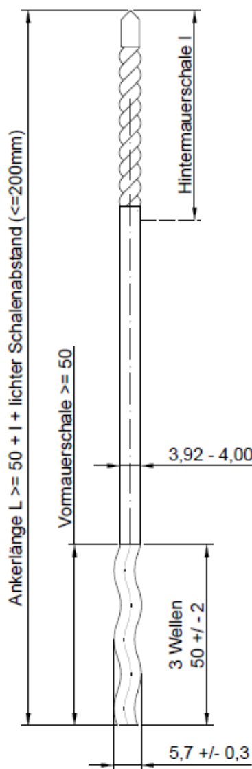
"Well-L-Form" (3 Wellen)
